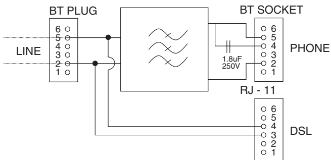
Z-350UK Block Schematic – includes a BT specified “Ringing Capacitor”
